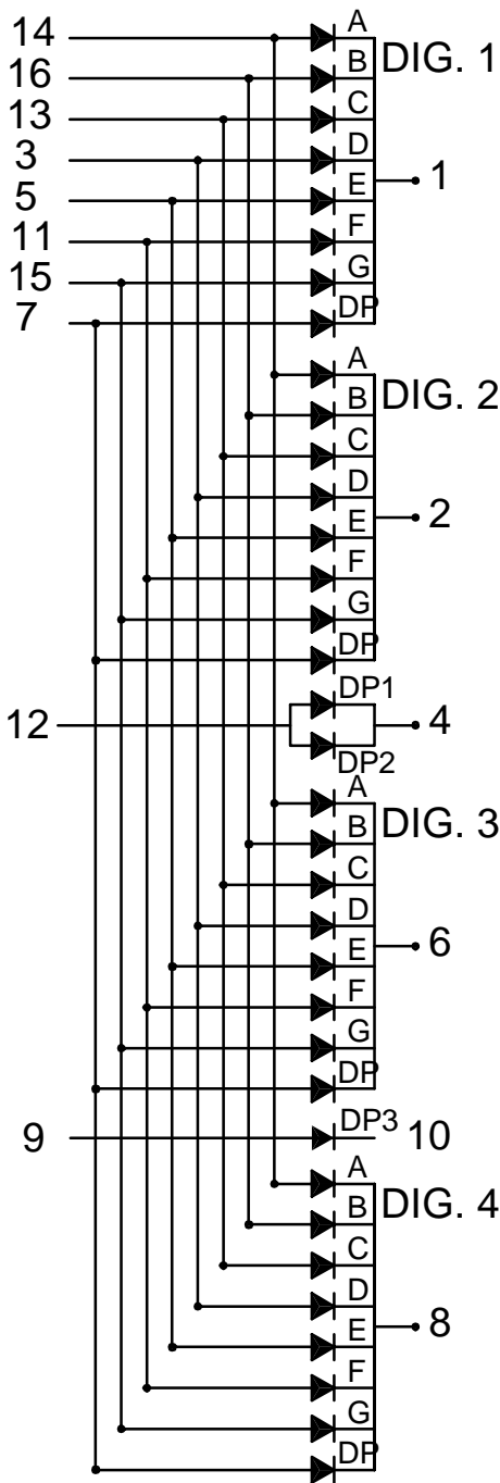
LFD4154-XX/SRP10-2-PF
