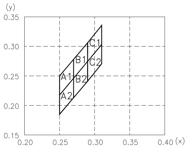
C.I.E. 1931 Chromaticity Diagram
