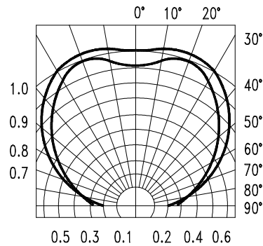
■ Directivity
