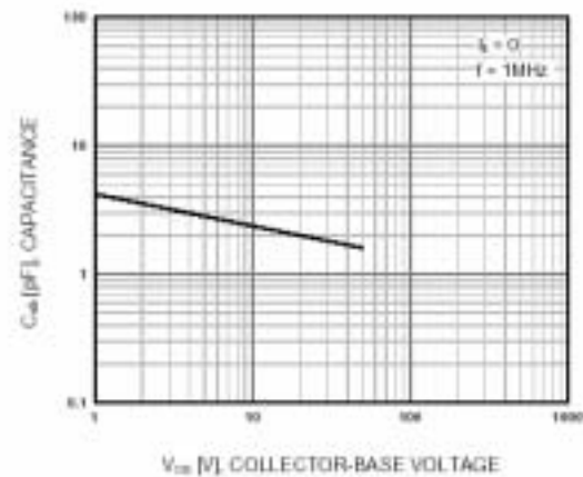
Figure 5. Output Capacitance
