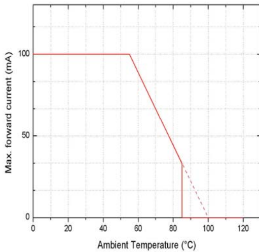
Ambient Temperature vs. maximal forward current
