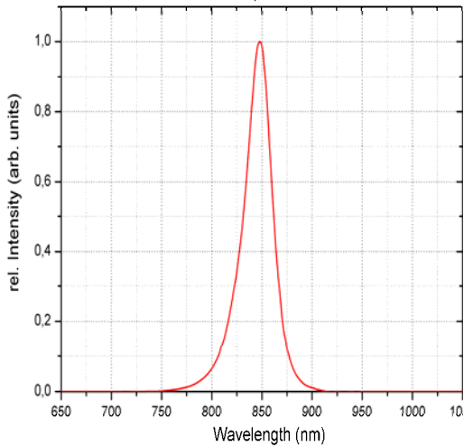
Spectral power distribution (typical) at I_F = 20 \text{ mA}
