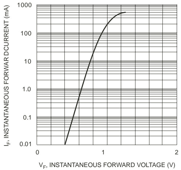
Fig. 2 Forward Characteristics
