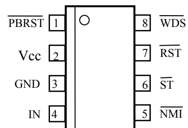
Fig. 2 – Pin assignment
