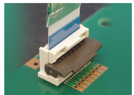
Vertical - Front View (Actuator Closed)
