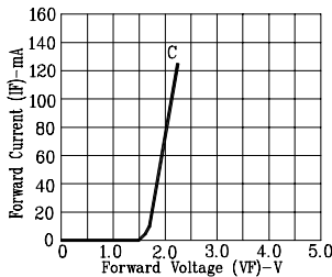
Fig3. FORWARD CURRENT VS. FORWARD VOLTAGE
