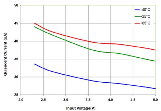
Figure 11 Quiescent Current
