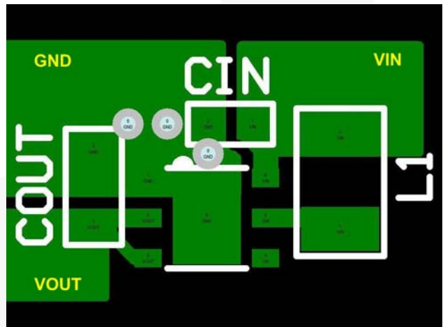
Figure 33 UMLP Suggested Layout (Top View)
