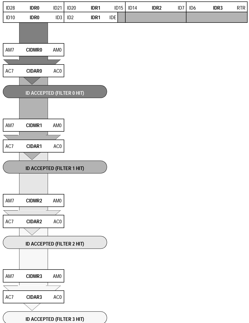
Figure 21-5. Quadruple 8-Bit Maskable Acceptance Filters
