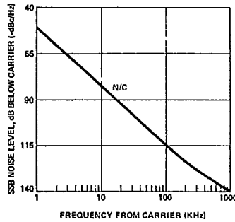
Figure 13. Typical Phase Noise to Carrier Ratio (N/C) vs. Frequency from Carrier at 4.3 GHz ( V_{CE} = 15 V, I_C = 30 mA), for the HXTR-4101.
