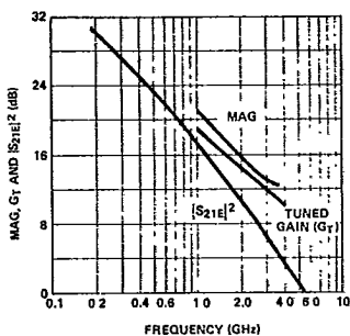
Figure 2. Typical MAG, |S 21E | 2 , and Tuned Gain vs. Frequency (V CE = 15 V, I C = 25 mA), for the HXTR-2101.
