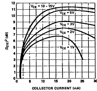
Figure 6. Typical |S 21E | 2 vs. Collector Current at 2 GHz, for the HXTR-2102.
