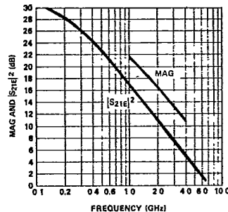
Figure 3. Typical MAG, and |S 21E | 2 vs. Frequency (V CE = 15 V, I C = 25 mA), for the HXTR-2102.
