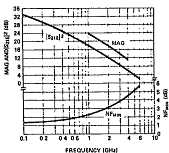
Figure 1. Typical MAG, |S 21E | 2 , and Noise Figure (NF MIN ) vs. Frequency (V CE = 15 V, I C = 25 mA), for the HXTR-2001.
