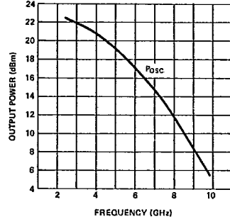
Figure 11. Typical Tuned Power Output vs. Frequency ( V_{CE} = 15 V, I_C = 30 mA) for the HXTR-4101.
