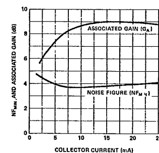
Figure 15. Typical NF_{MIN} and Associated Gain vs. Collector Current at 4 GHz for V_{CE} = 15 V (Tuned for NF_{MIN} ) for the HXTR-6105.
