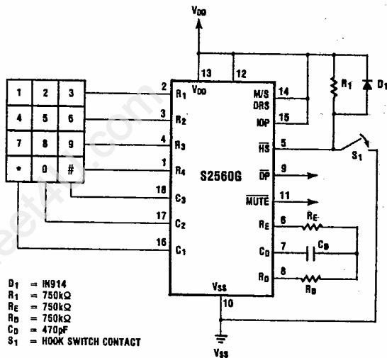
Figure 1. Transient Protection Technique Using Diode Between V_{DD} and \overline{HS}
