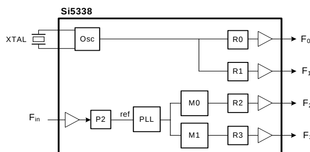
Figure 19. Si5338 In a Free-Running and Synchronous Clock Generator Application
