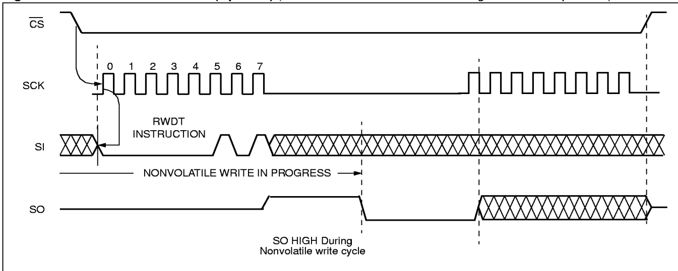
Figure 10. Read Nonvolatile Status (Option 2) (Used to determine end of Watchdog Timer store operation)
