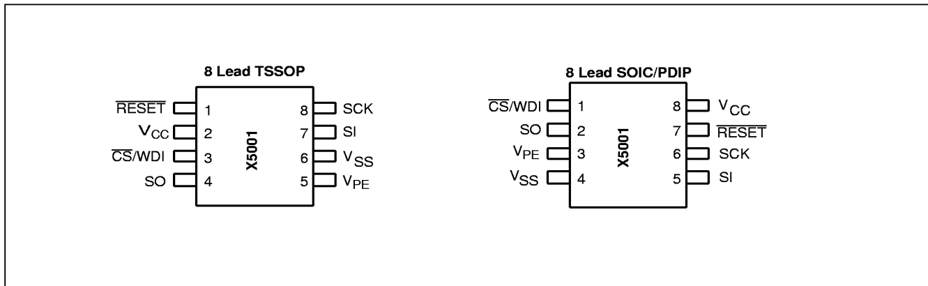
Figure 1. PIN CONFIGURATION
