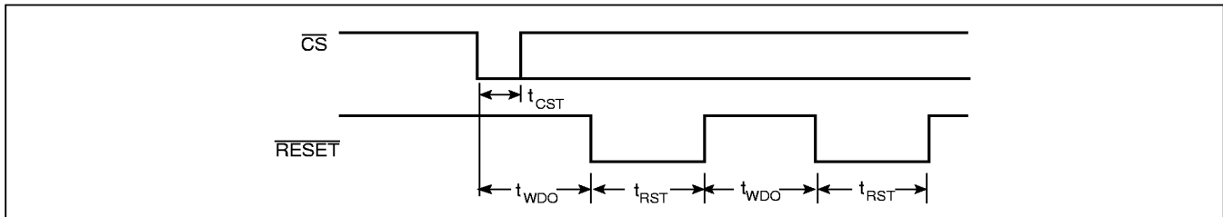
Figure 2. CS vs. RESET Timing
