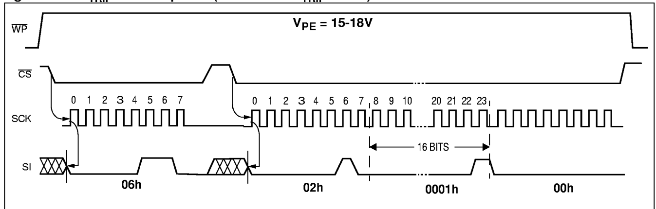
Figure 4. Reset V_{TRIP} Level Sequence ( V_{CC} > 3V .)
