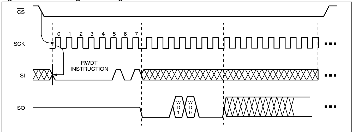
Figure 6. Read Watchdog Timer setting
