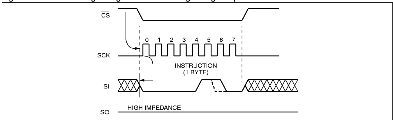
Figure 7. Enable Watchdog Change/Disable Watchdog Change Sequence
