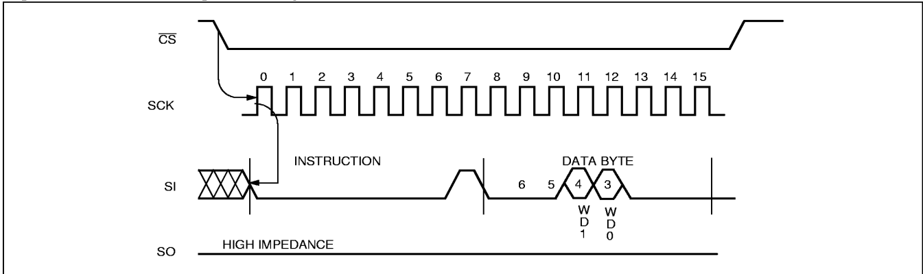
Figure 9. Read Nonvolatile Status (Option 1) (Used to determine end of Watchdog Timer store operation)
