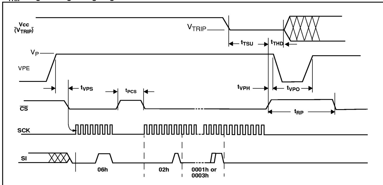
V TRIP Programming Timing Diagram
