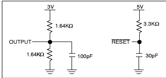
Figure 1. EQUIVALENT A.C. LOAD CIRCUIT
