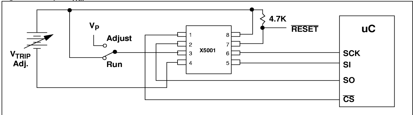
Figure 3. Set V_{TRIP} Level Sequence ( V_{CC} =desired V_{TRIP} value.)
