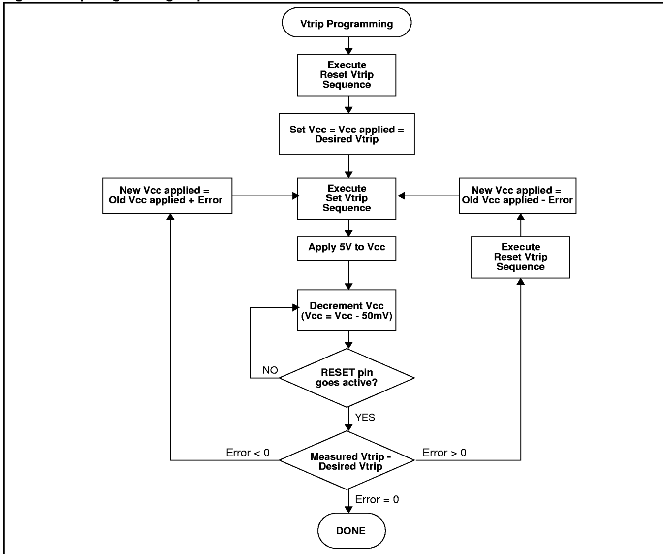
Figure 5. Vtrip Programming Sequence
