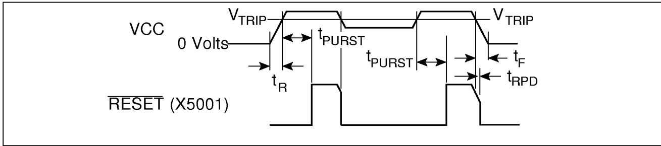
Figure 1. Power-Up and Power-Down Timing
