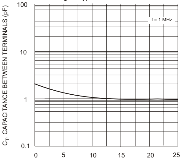
V_R , REVERSE VOLTAGE (V) Fig. 3 Typical Capacitance Between Terminals Characteristics
