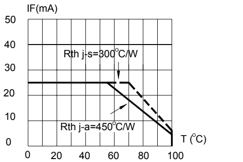
FIG.5 MAXIMUM FORWARD DC CURRENT VS TEMPERATURE. DERATING BASED ON Tjmax=110°C
