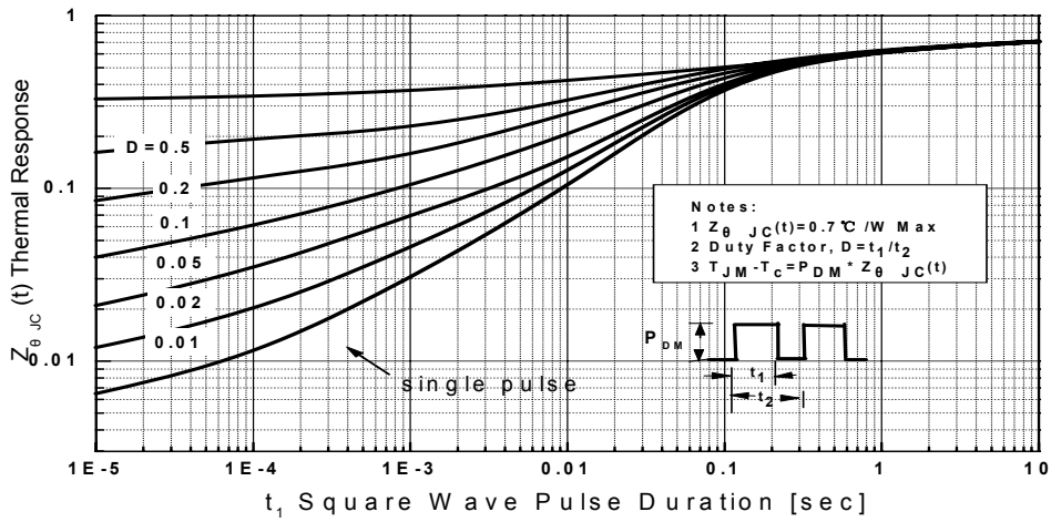
Transient Thermal Response Curve For JCS10N65CT
