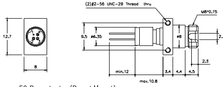
FC Receptacle (Board Mount)
