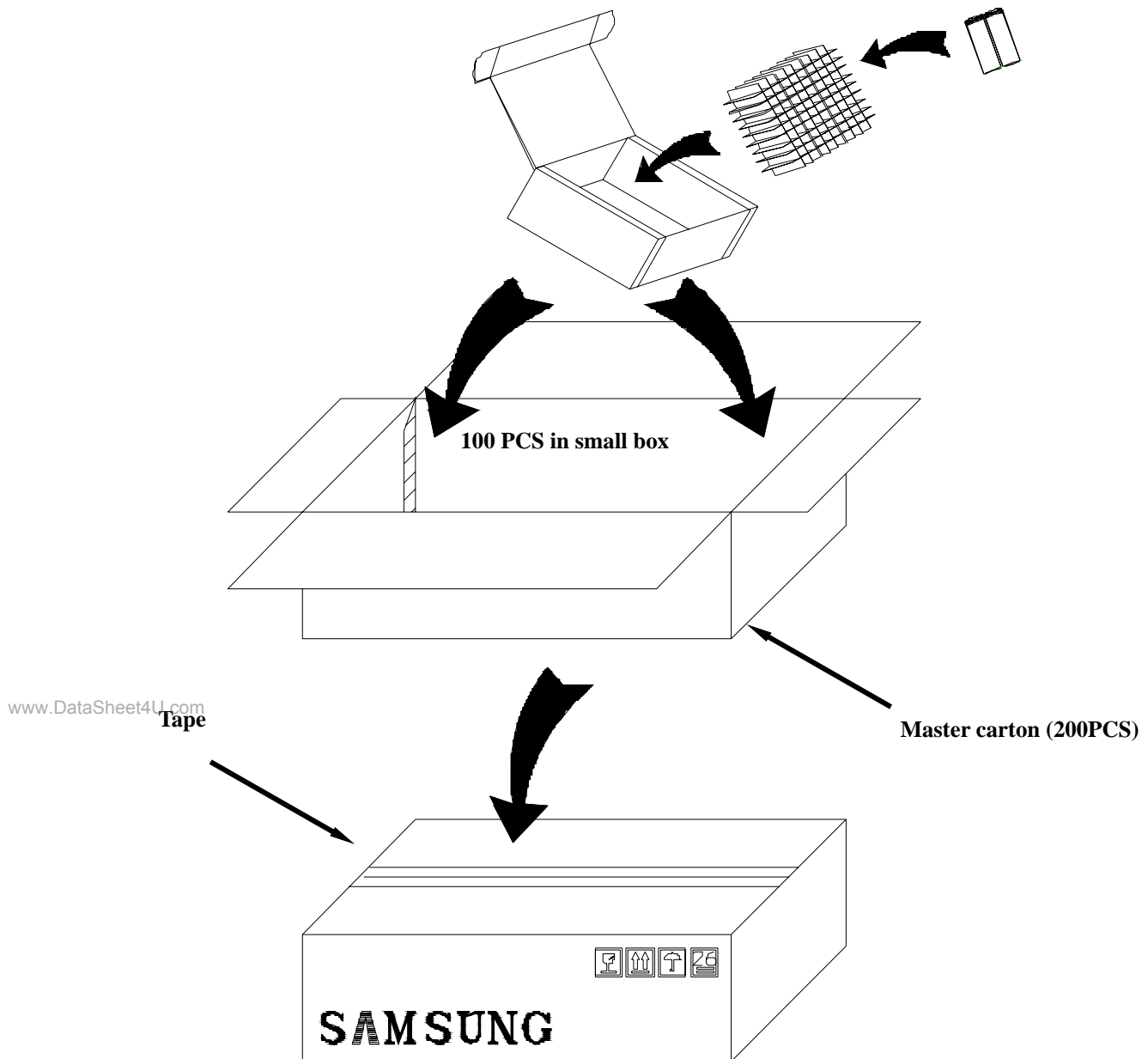
Fig.2. Package Drawing
