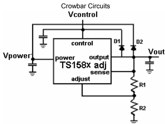
Figure 6. Optional Clamp Diodes Protect Against Input
