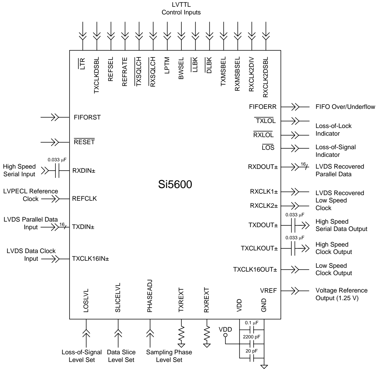
Figure 4. Si5600 Typical Application Circuit
