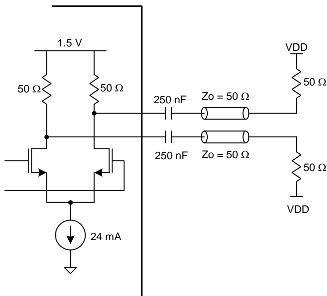
Figure 5. CML Output Driver Termination (TXCLKOUT, TXDOUT)
