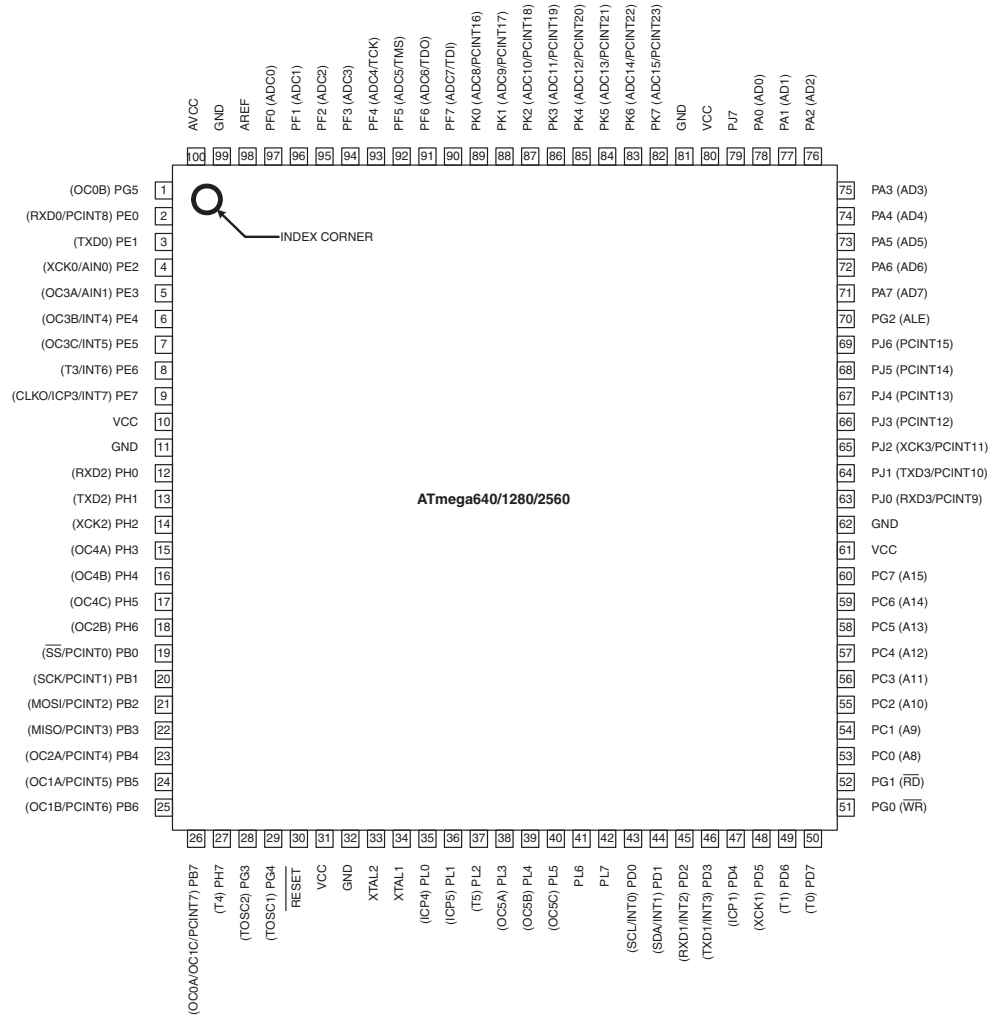
Figure 1. TQFP-pinout ATmega640/1280/2560
