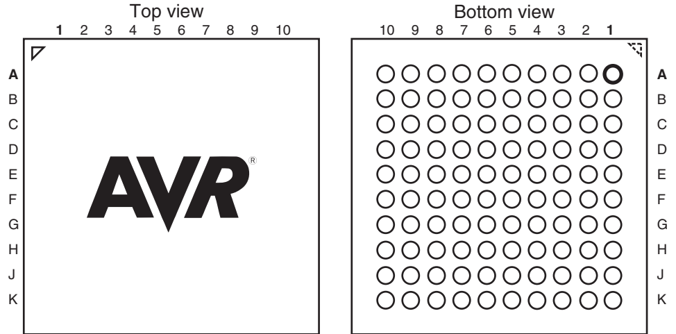
Figure 2. CBGA-pinout ATmega640/1280/2560
