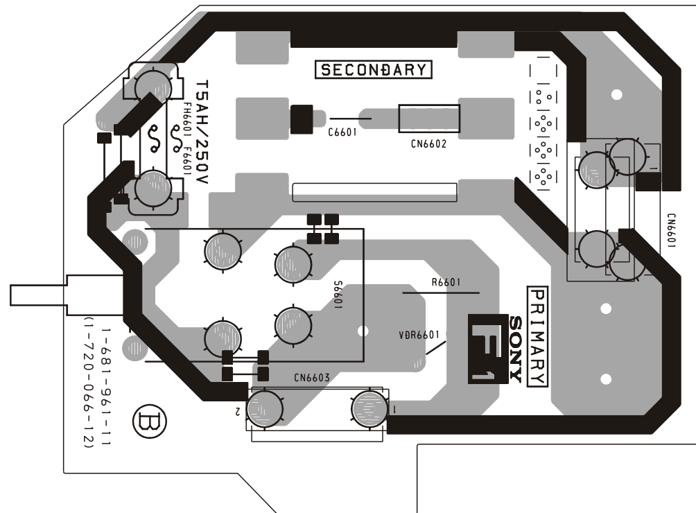
F1 [ AC FILTER, FUSE, SIRCS ]
