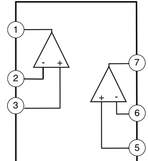
A BOARD IC401/IC531 LM393DT
