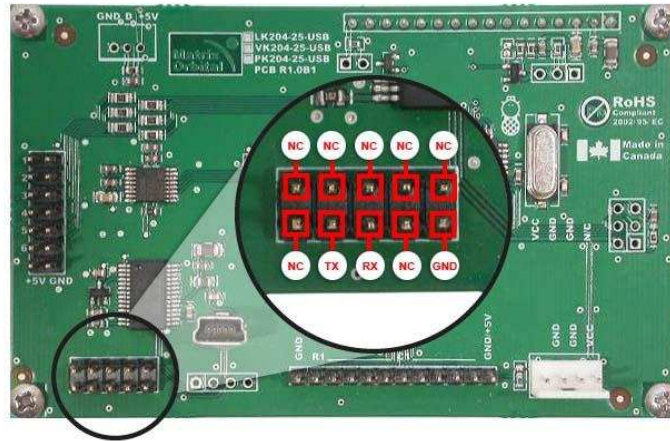
Figure 12: Serial Header
