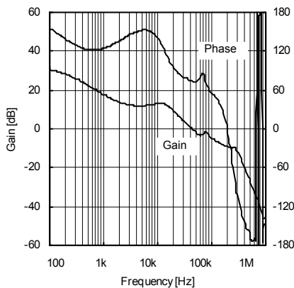
Fig.30 Frequency response property 5 (VCC = 6.0 V, Io = 500 mA)
