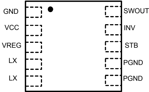
Fig.1 Pin layout
