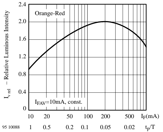
Figure 7. Rel. Luminous Intensity vs. Forw. Current/Duty Cycle
