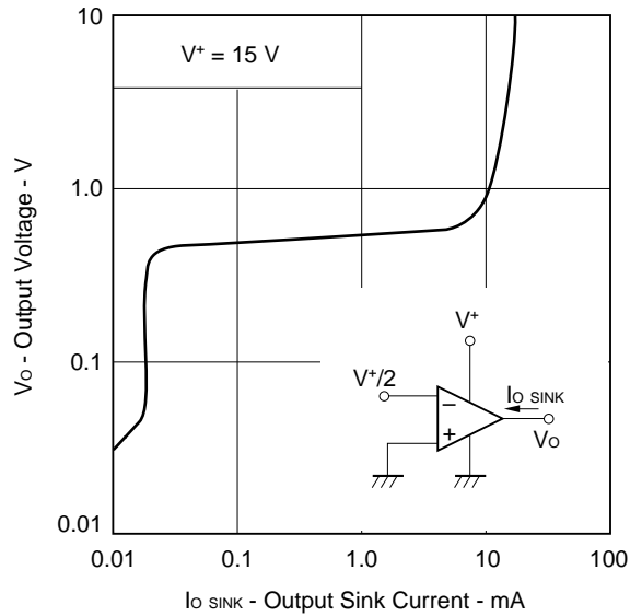
OUTPUT SINK CURRENT LIMIT
