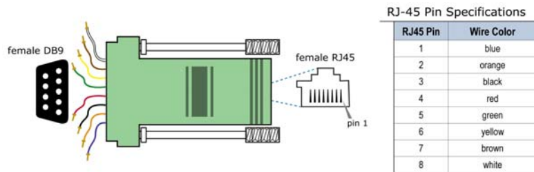
Figure B-6. Female DB-9 to RJ-45 Adapter and pinouts
