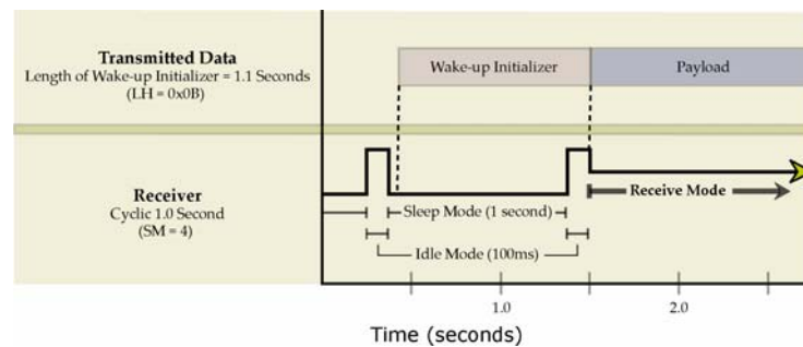
Figure 3-07. Correct Configuration (LH > SM):
