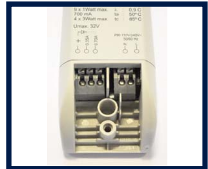
Input and output clamps
