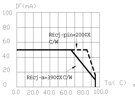
FIG.5 MAXIMUM FORWARD DC CURRENT VS TEMPERATURE. DERATING BASED ON T_{jmax} = 110^\circ C
