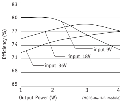
Figure 7 : Typical efficiency versus load at various input
