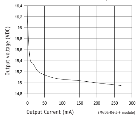
Figure 12 : Typical load regulation characteristics at nominal input
