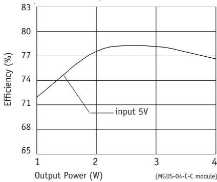
Figure 4 : Typical efficiency versus load at various input
