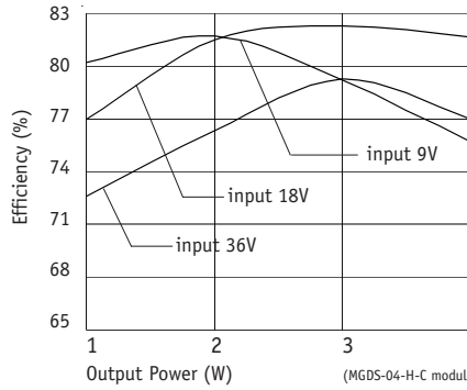
Figure 8 : Typical efficiency versus load at various input
