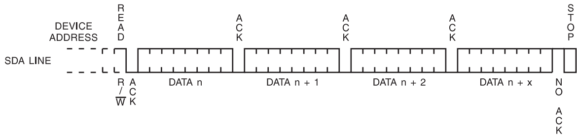
Figure 13. Sequential Read
