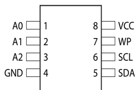
8-lead TSSOP
