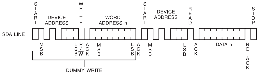
Figure 12. Random Read
