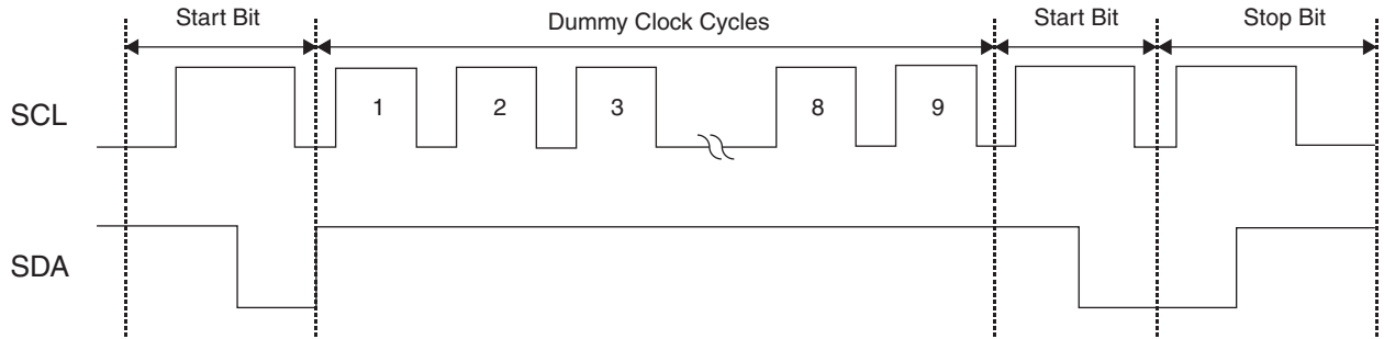
Figure 2. Software Reset
