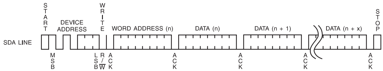
Figure 10. Page Write
