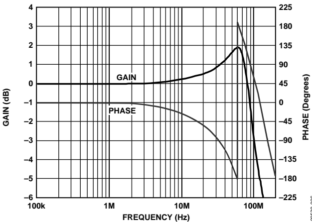
Figure 6. Frequency and Phase Response vs. Gain (Gain = -10\text{ dB} , P_{IN} = -30\text{ dBm} )
