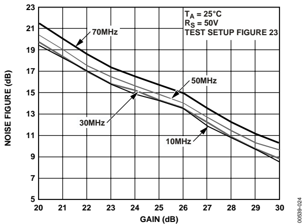
Figure 24. Noise Figure in -10 dB/+30 dB Mode
