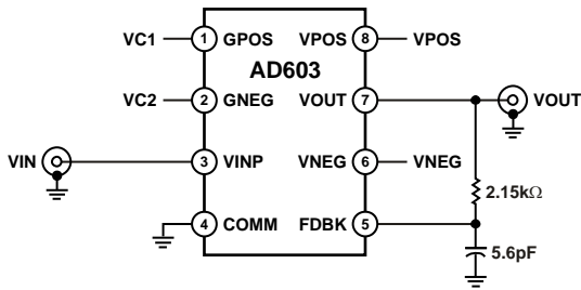
Figure 31. 0 dB to 40 dB; 30 MHz Bandwidth
