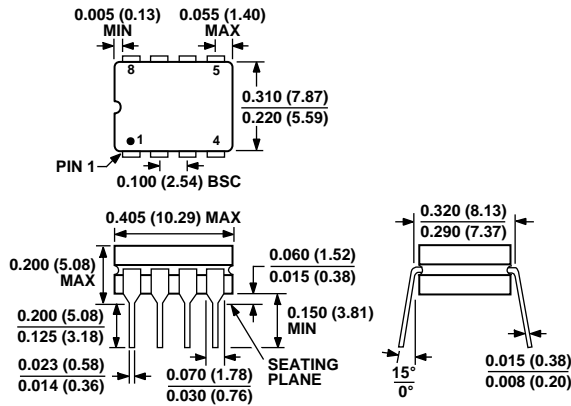
Figure 48. 8-Lead Ceramic Dual In-Line Package [CERDIP]
