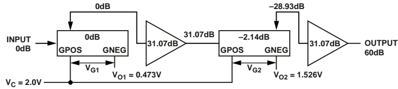
Figure 38. AD603 Gain Control Input Calculations for Sequential Operation V_C = 2.0\text{ V}
