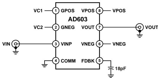
Figure 32. 10 dB to 50 dB; 9 MHz to Set Gain
