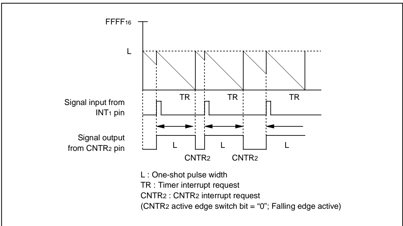
Fig. 32 Timing chart of programmable one-shot generating mode ("H" one-shot pulse generating)
