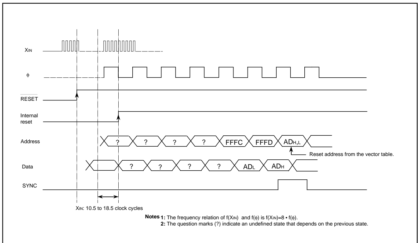
Fig. 58 Reset sequence
