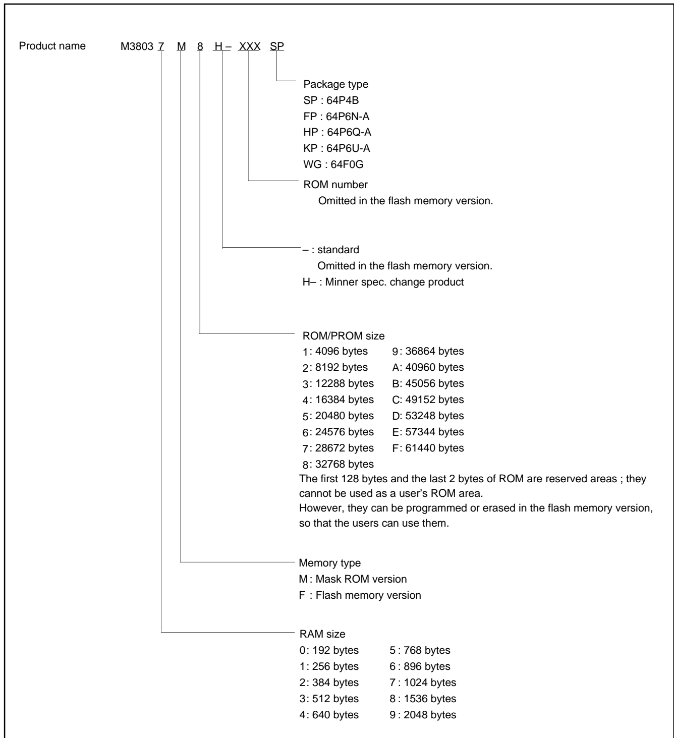
Fig. 5 Part numbering
