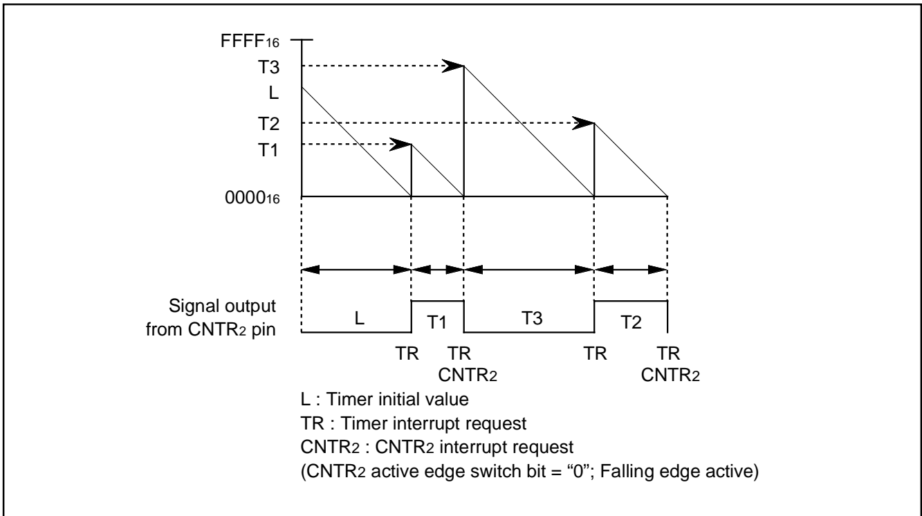
Fig. 31 Timing chart of programmable waveform generating mode
