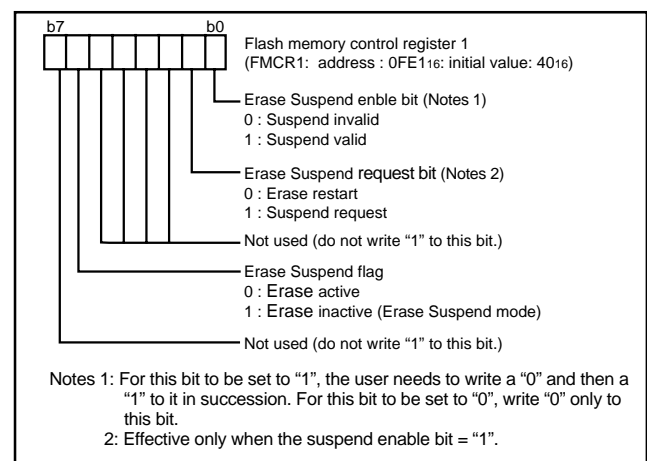
Fig. 66 Structure of flash memory control register 1
