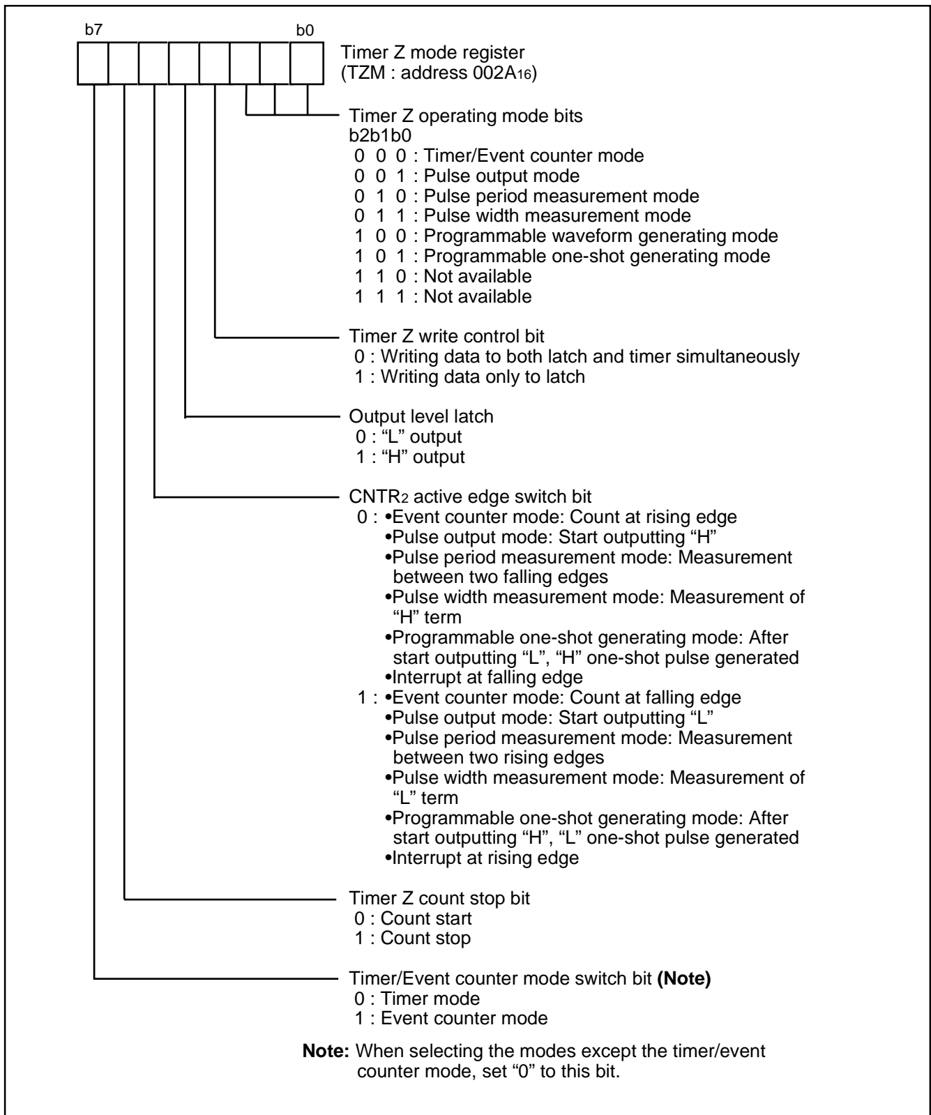
Fig. 26 Structure of timer Z mode register
