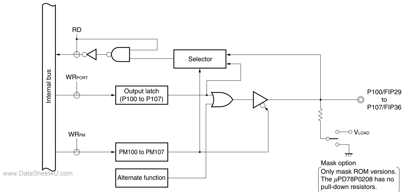
Figure 4-11. Block Diagram of P100 to P107
