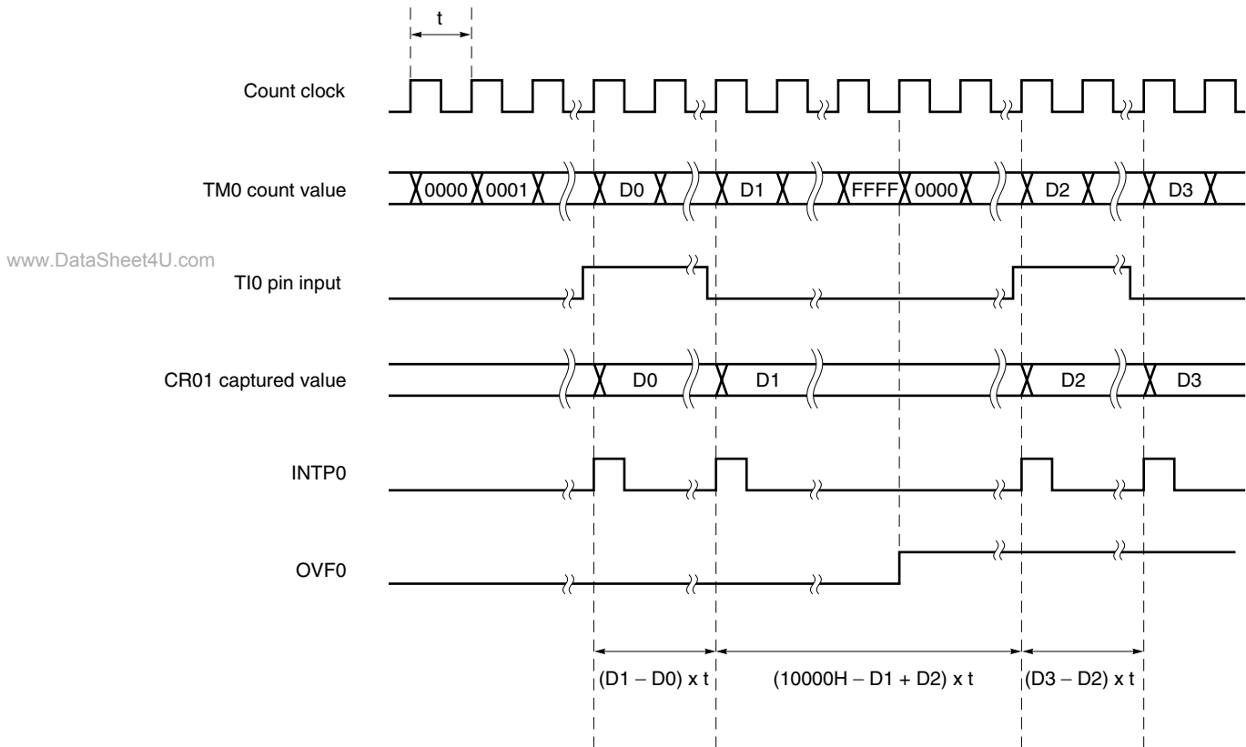
Figure 6-15. Timing of Pulse Width Measurement Operation in Free-Running Mode (with Both Edges Specified)
