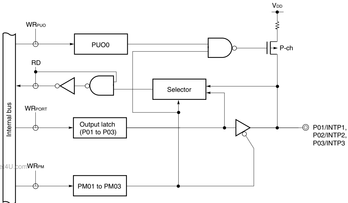
Figure 4-3. Block Diagram of P01 to P03
