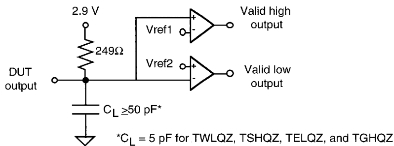
Tester Equivalent Load Circuit
