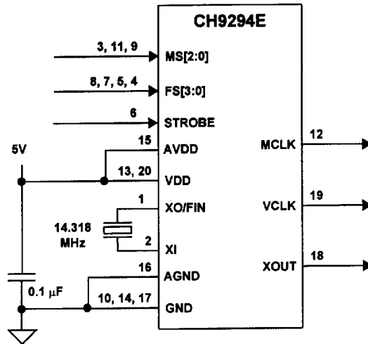
Figure 4: Application Schematic
