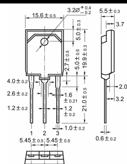
TO-3PFM
