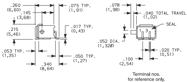
GP11MSA1BE SPST
