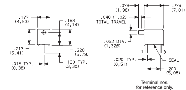
GP11MCBE SPST
