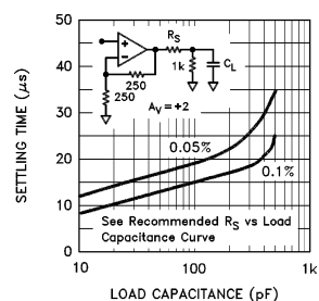
Settling Time vs Load Capacitance
