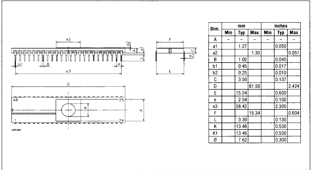
Figure 5. 48-Pin Window Dual In Line Ceramic Multilayer (D), 600-Mil Width
