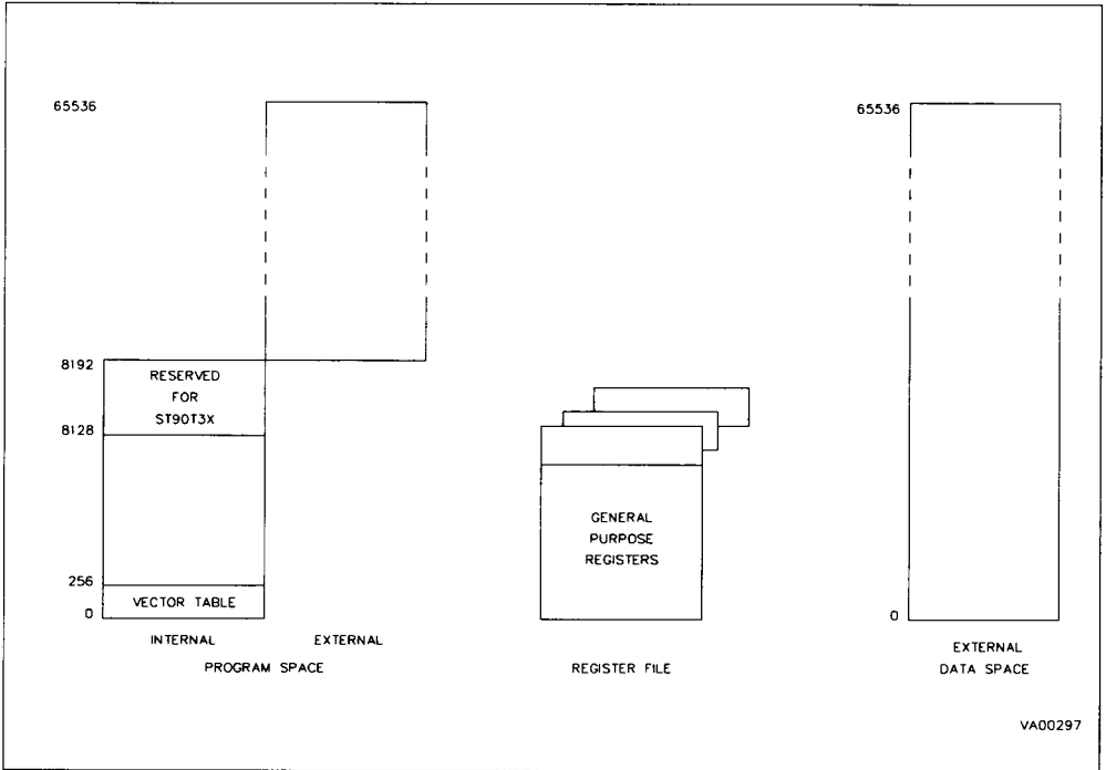
Figure 4. Memory Spaces
