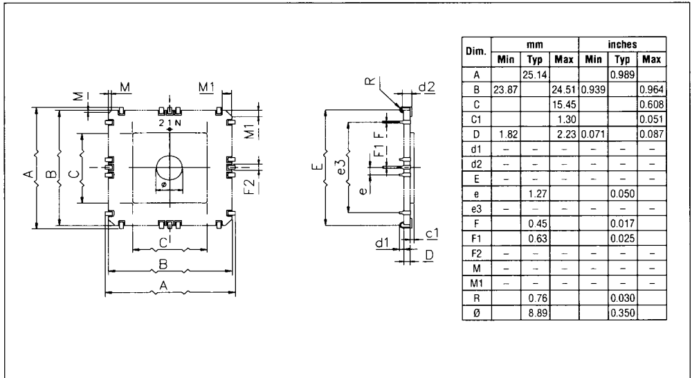
Figure 6. 68-Lead Window Ceramic Leaded Chip Carrier (L)
