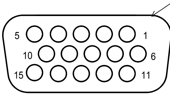
D-sub connector
