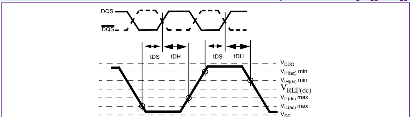
Differential input waveform timing - t_{\text{DS}} and t_{\text{DH}}
