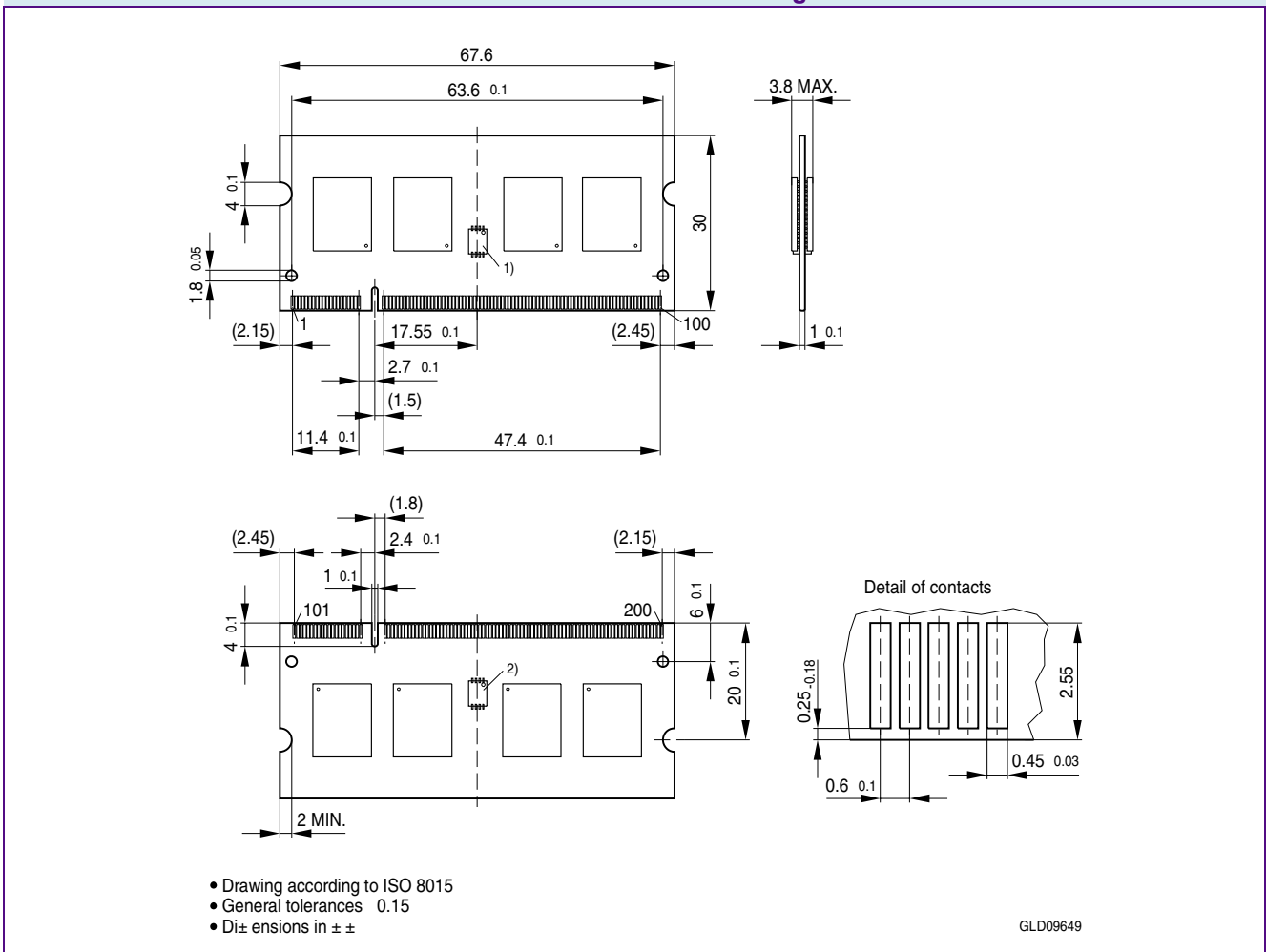
FIGURE 5 Package Outline Raw Card A LG-DIM-200-31
