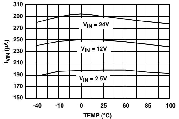
FIGURE 5. V_{IN} CURRENT
