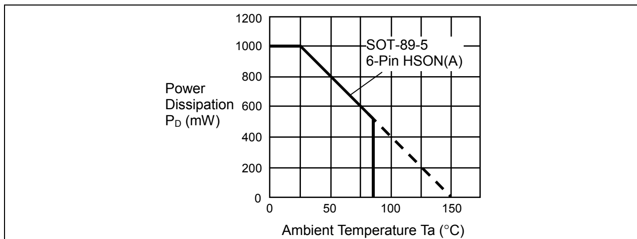
Figure 4 Power Dissipation of Package (Mounted on Printed Circuit Board)
