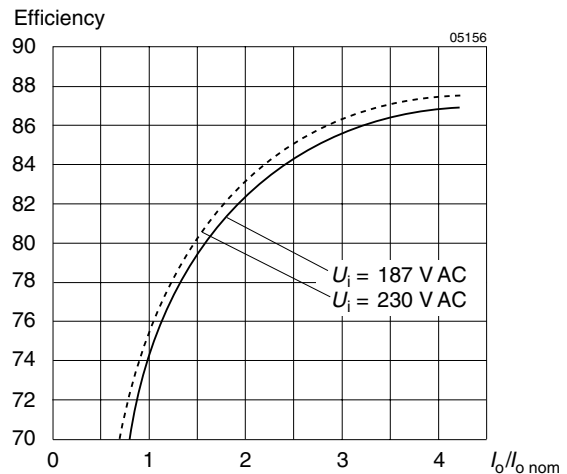
Fig. 8 Efficiency versus load at U_i 230 V AC and 187 V AC
