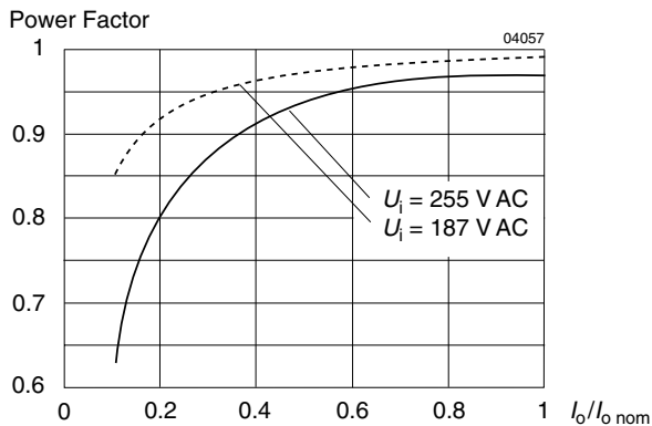
Fig. 4 Power factor versus output power at U_i 255 V AC and 187 V AC.
