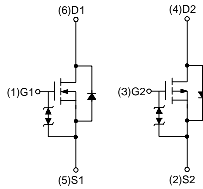
N-Channel MOSFET
