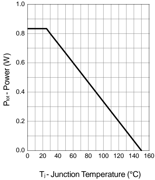
Power Dissipation
