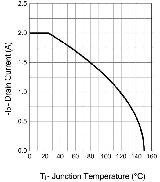
Drain Current
