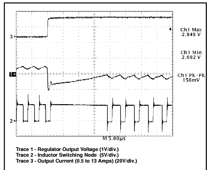
Figure 8: CS-5155 demonstration board response to 13A load turn on (output set for 2.8V). Upon completing a normal off time, the V^{2TM} control loop immediately connects the inductor to the input voltage, providing 100% duty cycle. Regulation is achieved in less than 20µs.
