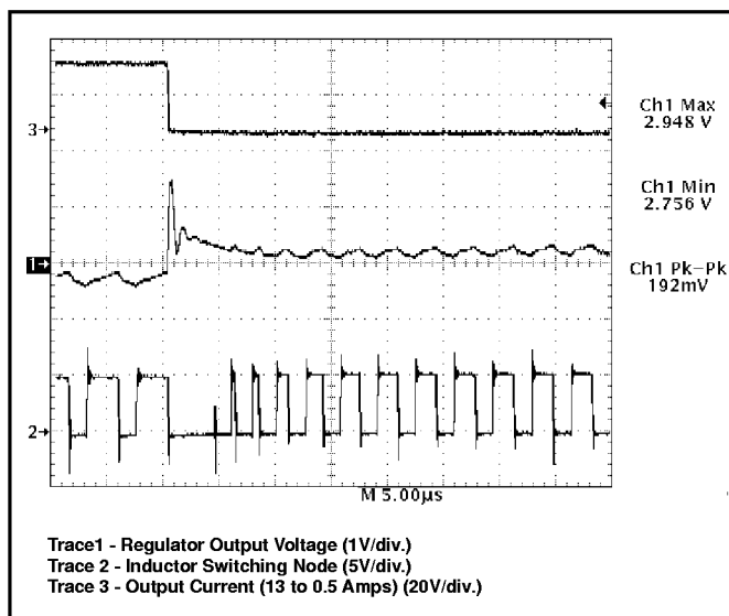
Figure 9: CS-5155 demonstration board response to 13A load turn off (output set for 2.8V). V 2 ™ control topology immediately connects inductor to ground, providing 0% duty cycle. Regulation is achieved in less than 10µs.
