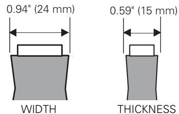
Maximum dimensions of the HDMI connectors
