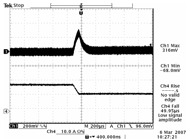
75%-50% Load Transients
