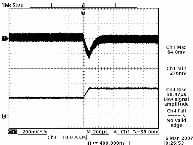
50%-75% Load Transients
