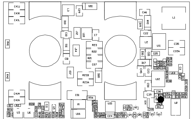
The thermistor on the bottom side: R25
