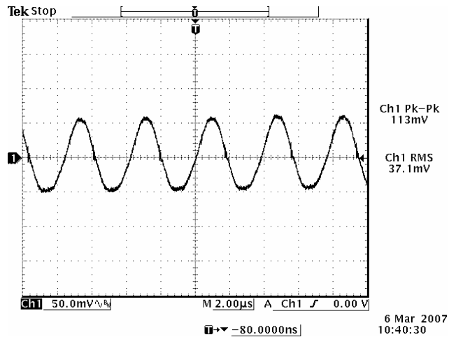
48 Vdc input, 12Vdc/25A output
